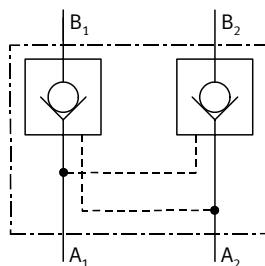
Pilot-operated double non-return valve
