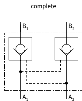
Piloted double non-return valve, symbol
